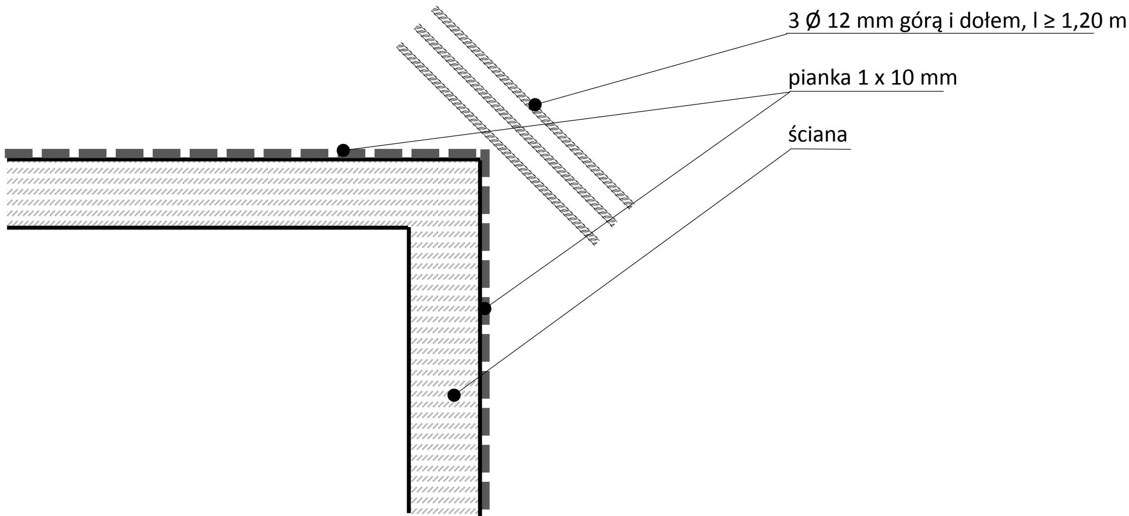
re-entering corner
