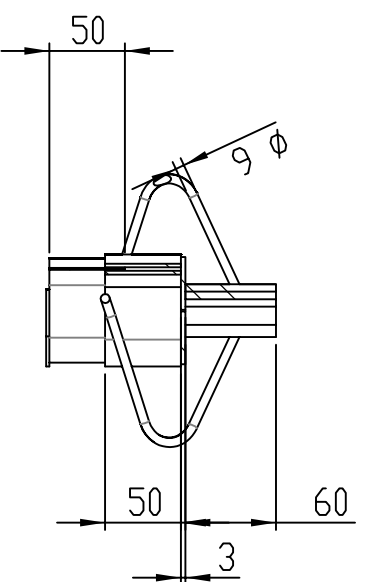
SECTION C-C SCALE 1 : 5
